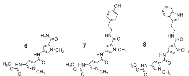
Figure 2. Structures of the synthetic netropsin–proximicin hybrids A ( 6 ), B ( 7 ), and C ( 8 ).
