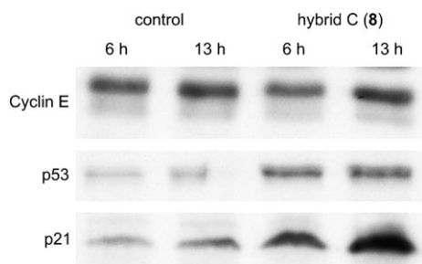
Figure 3. Western blot analysis showing the effect of netropsin–proximicin hybrid C ( 8 ) on the upregulated expression of p21, p53, and cyclin E in AGS cells after 6 h and 13 h incubation.
