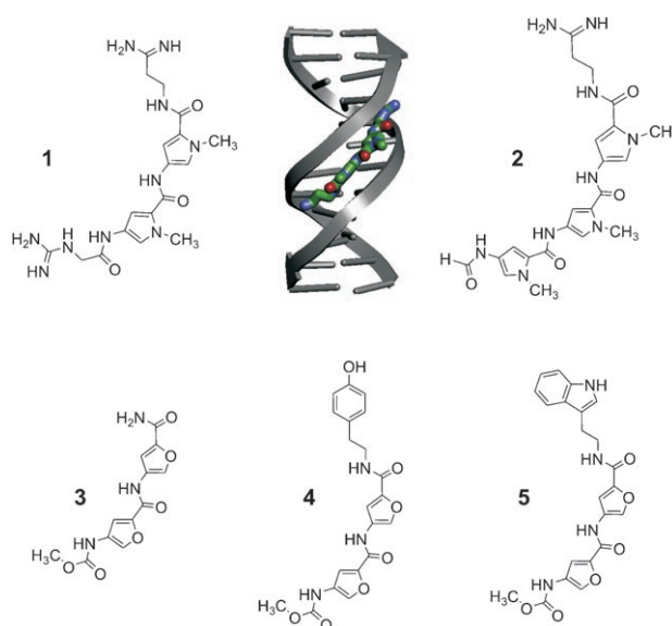
Figure 1. Structures of netropsin ( 1 ), distamycin ( 2 ), and of the compounds from the marine Verrucosisspora : proximicin A ( 3 ), proximicin B ( 4 ), and proximicin C ( 5 ). The double helix illustrates the binding of netropsin ( 1 ) in the minor groove of DNA to form a 1:1 complex. [13]
